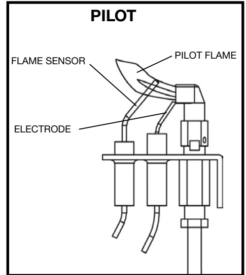
Figure 73: Pilot assembly.
