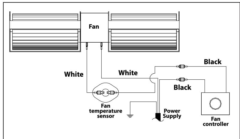
Figure 51: Wiring Diagram For Fan Control.
