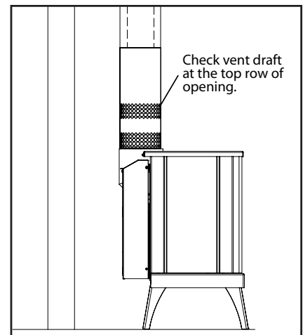
Figure 47: Draft test place.
