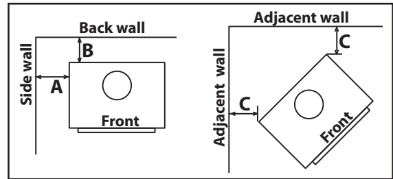
Figure 17: Clearances to combustibles.
