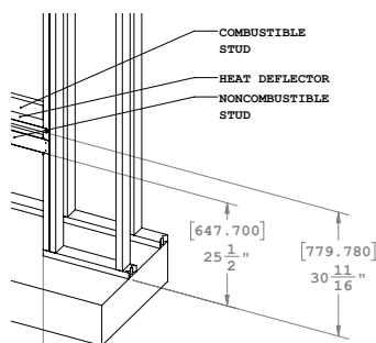
DRL*6013 DIMENSIONS
