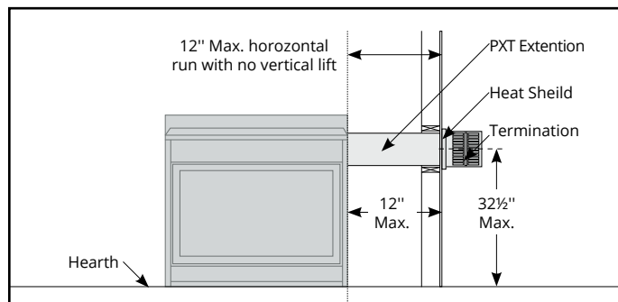
Figure 8. Straight run, Side Vented, wall mounted termination for H*38DF*-ST
