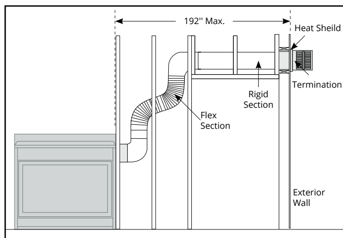
Figure 8. Side Vented, wall mounted Multi-elbow installation
