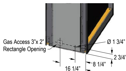
Figure 18.b Gas Inlet Supply location (left side shown)
