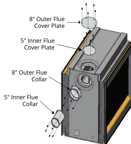
Figure 5.b Flue cover and collar installation, Side Vented fireplace.
