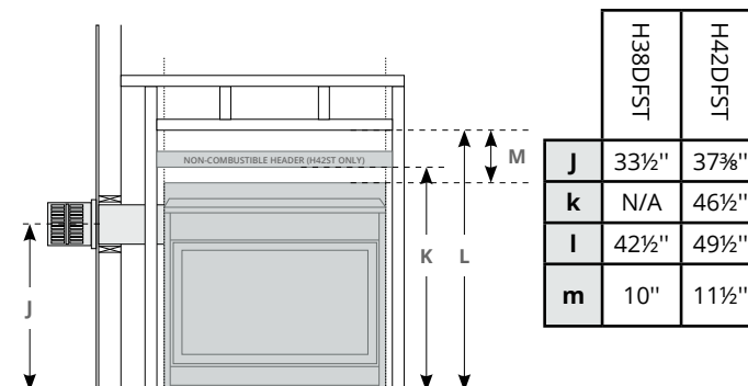
Figure 3.b Combustible Framing for shelves over the fireplace, Side vent.
