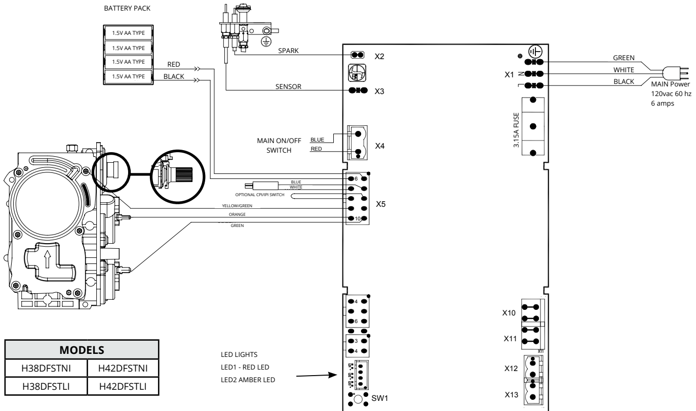
Figure 16. Wiring diagram for SIT Proflame 2 Electronic Ignition
