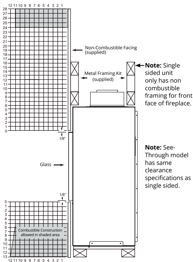
Figure 19. Combustible mantels and facings. (Not to scale)
