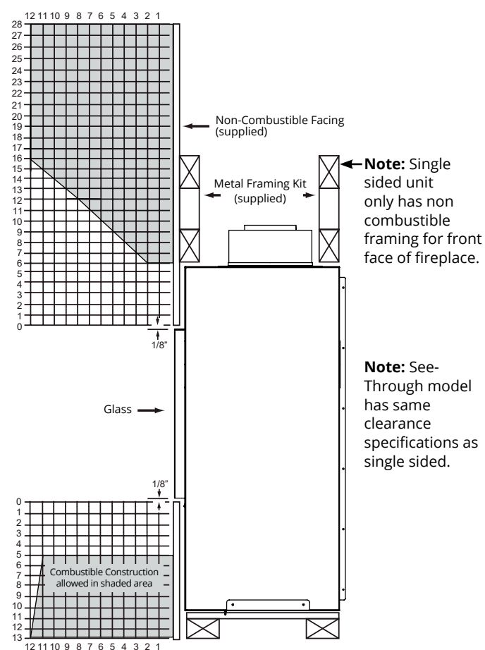
Figure 19.b Combustible mantels and facings with Cool Wall Kit. (Not to scale)
