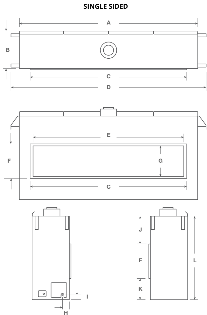
Figure 2. Distinction Fireplace dimensions (Tolerance \pm \frac{1}{8} ").
