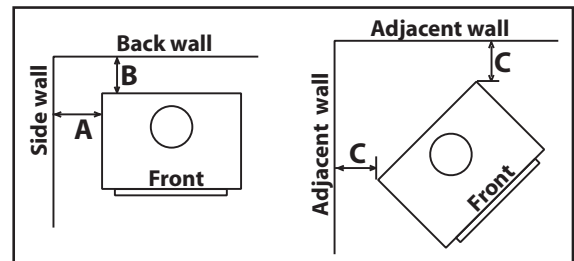
Figure 16: Clearances to combustibles.
