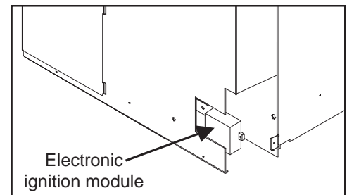
Figure 5: Electronic Ignition Module Location.
