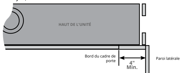
Figure 19.c Sidewall clearances
