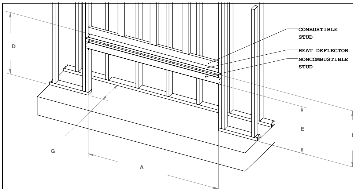
DRL*6013 DIMENSIONS
