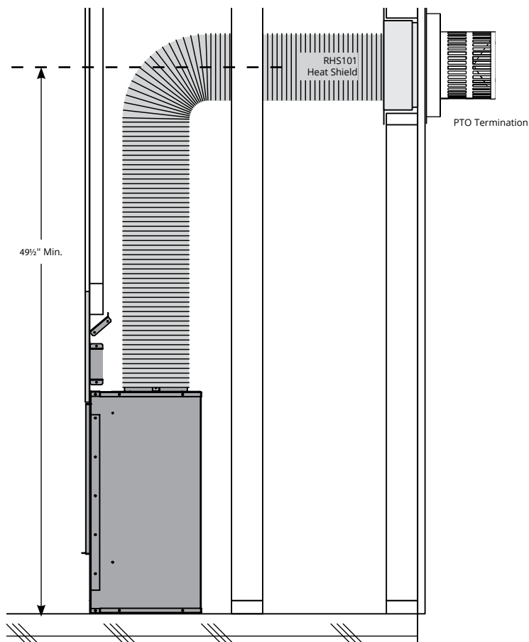
Figure 15.b RHS101 Installation. (Minimum requirements).
