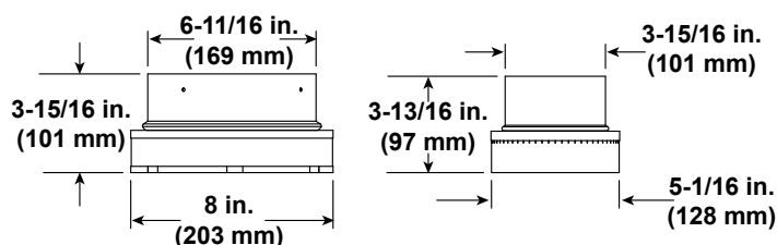
SLP-2DVP Adapter
