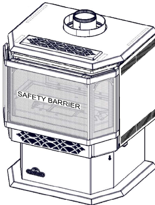
Model GS28 is made up of Model GDS28 and Natural Vent Adapter Kit GS-150KT
