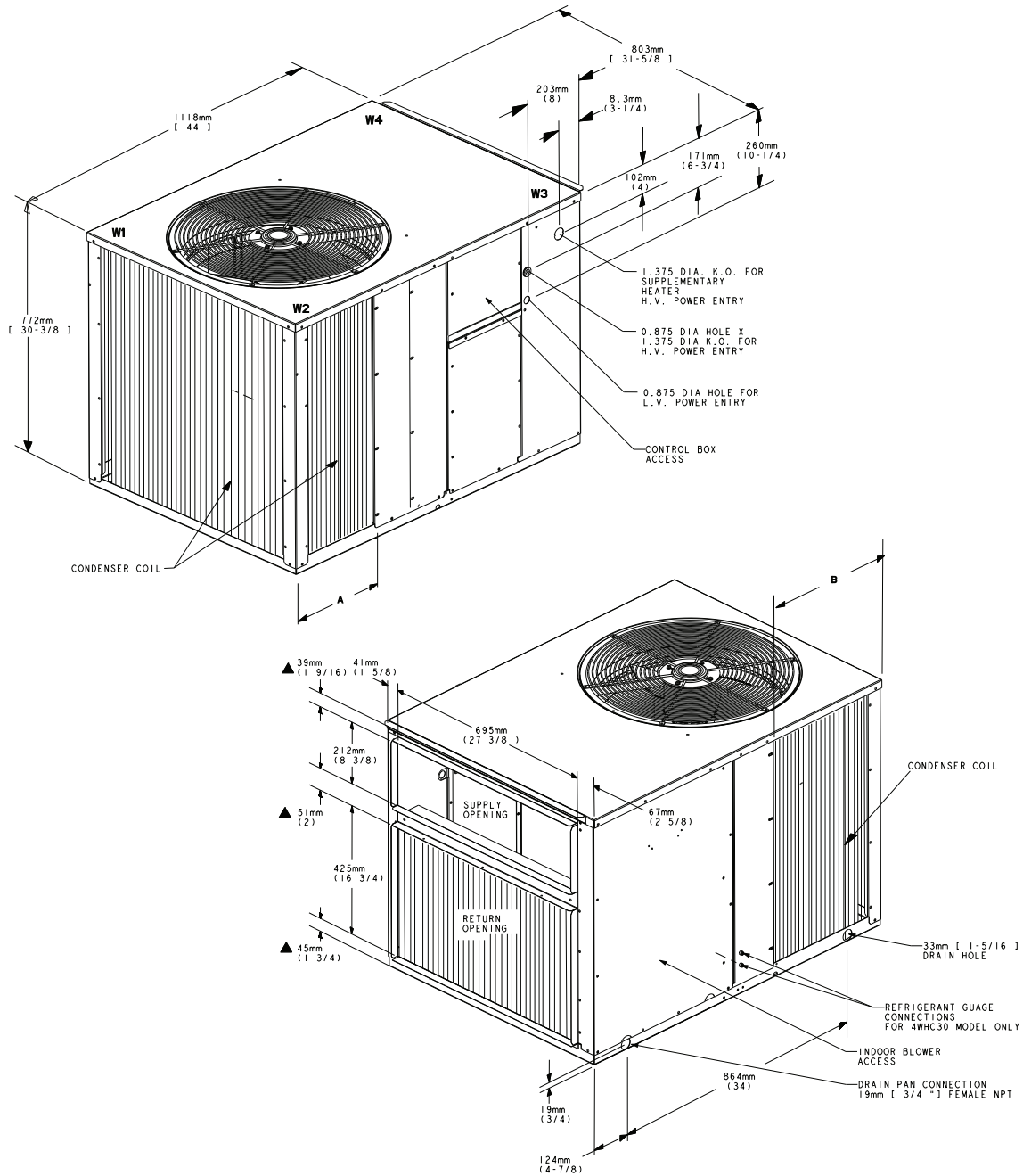
Figure 2. Outline Drawing
