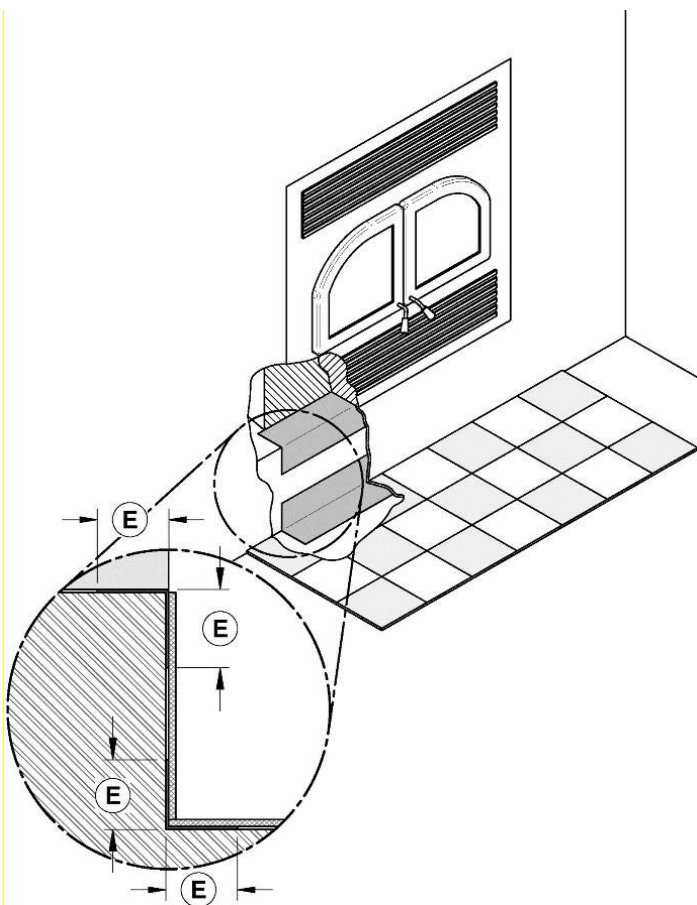
Figure 14 : Raised base installation of more than 4"
