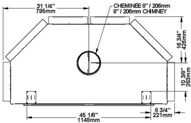
Figure 1 : Top View
