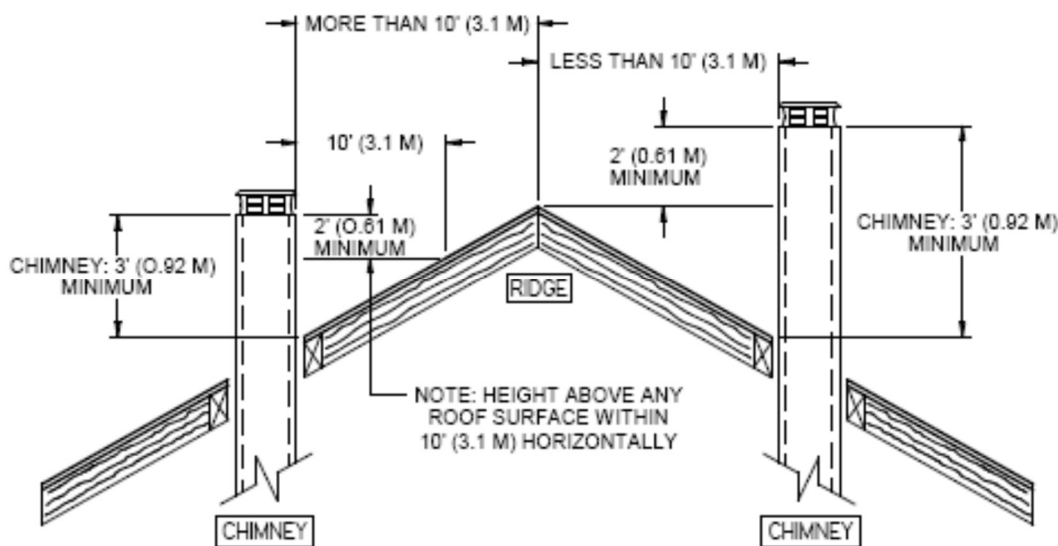
Figure 42 : Slope Roof
