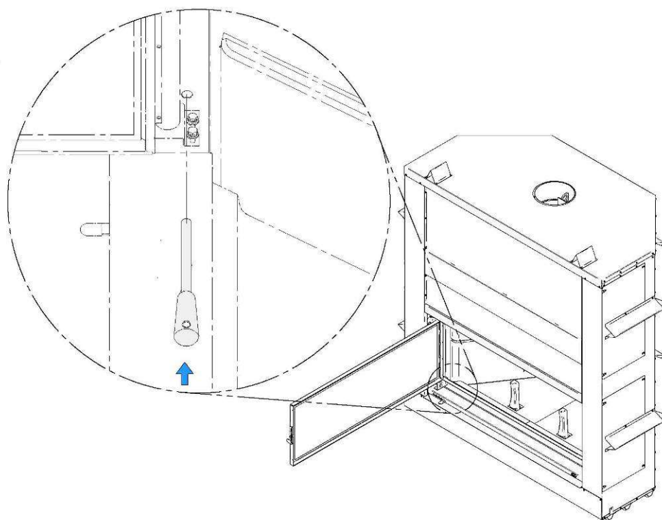
Figure 57 : Removable handle
