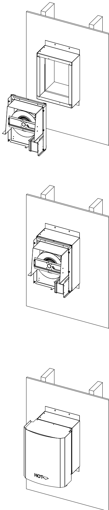
FIGURE 2.10 HTK-EXT FEK Install
