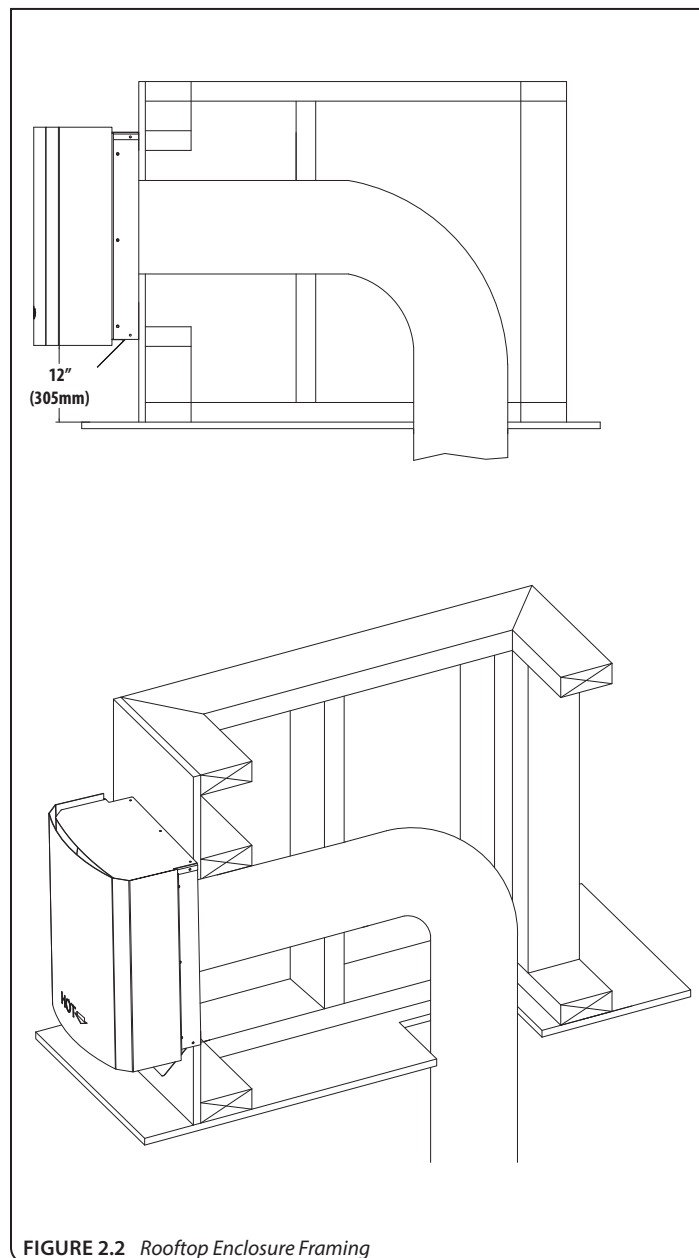
FIGURE 2.2 Rooftop Enclosure Framing
