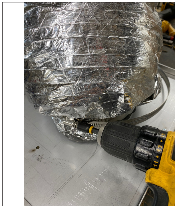
FIGURE 2.15 Liner Installed with Band Clamp
