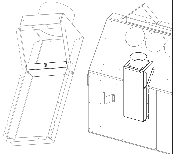
FIGURE 2.12 Air Chute Installation
