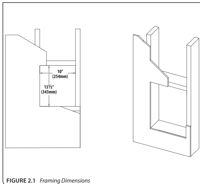
FIGURE 2.1 Framing Dimensions
