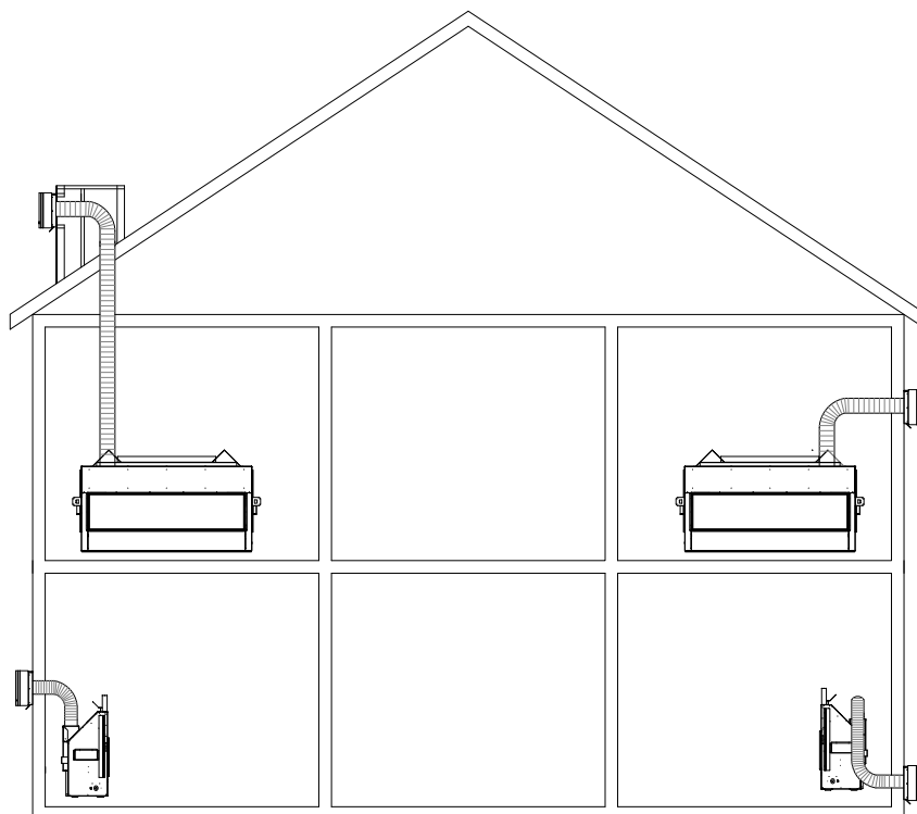
FIGURE 1.1 Possible Air Duct Locations/Terminations
