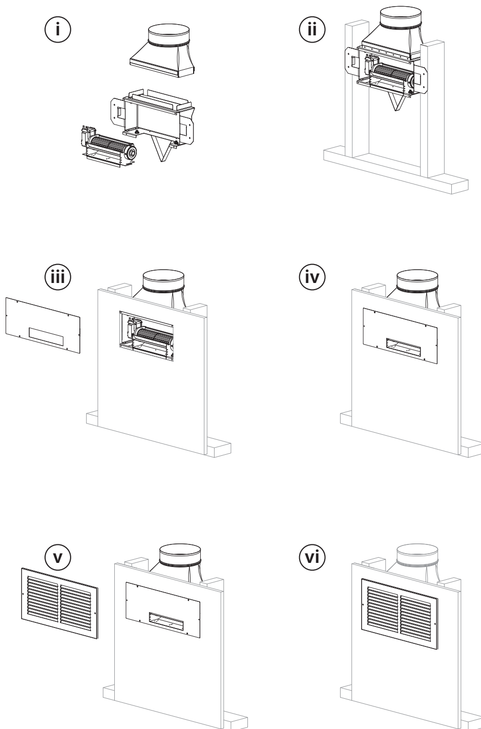
FIGURE 2.5 Fan Assembly Installation
