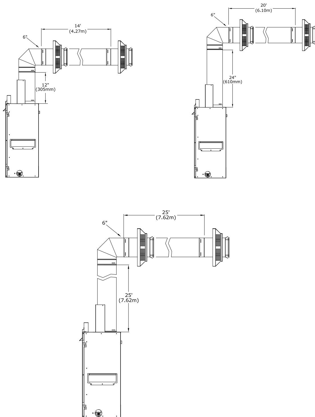
Figure 7.7 - Tuyau de ventilation horizontal 4" x 6-5/8"
