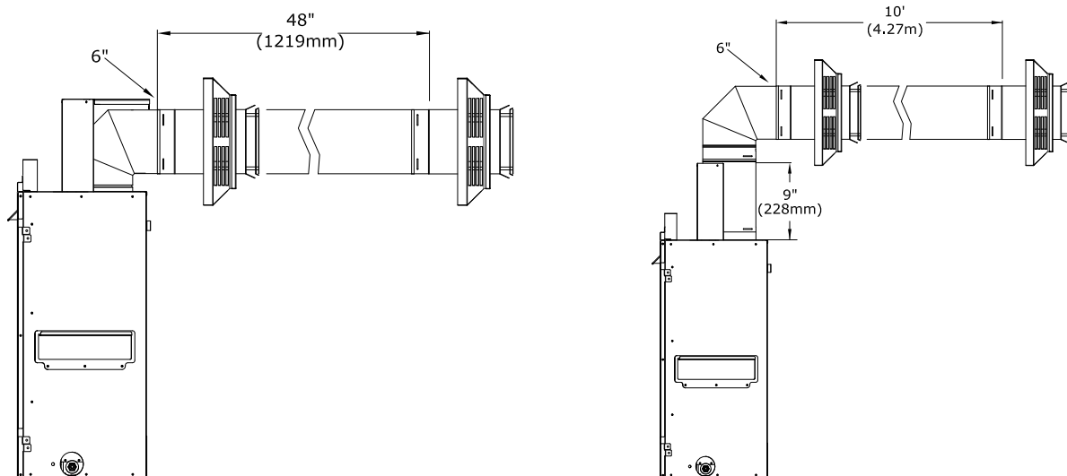
Figure 7.6 - Tuyau de ventilation horizontal 4" x 6-5/8"
