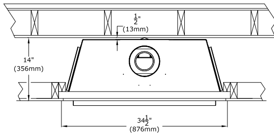
Installation verticale typique
