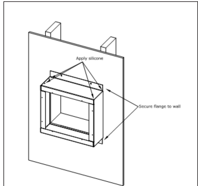
Figure 5.1 - Install FEK and Seal FEK
