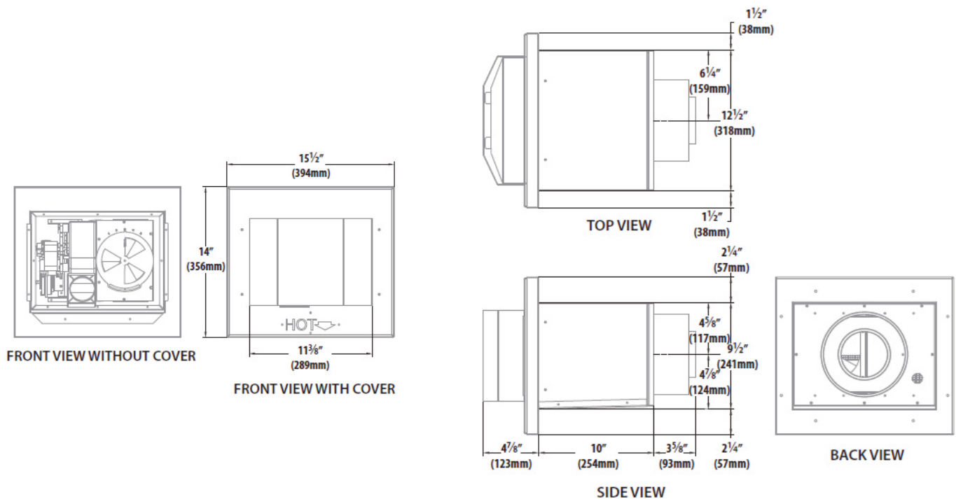
Figure 1.1 - KPV Dimensions
