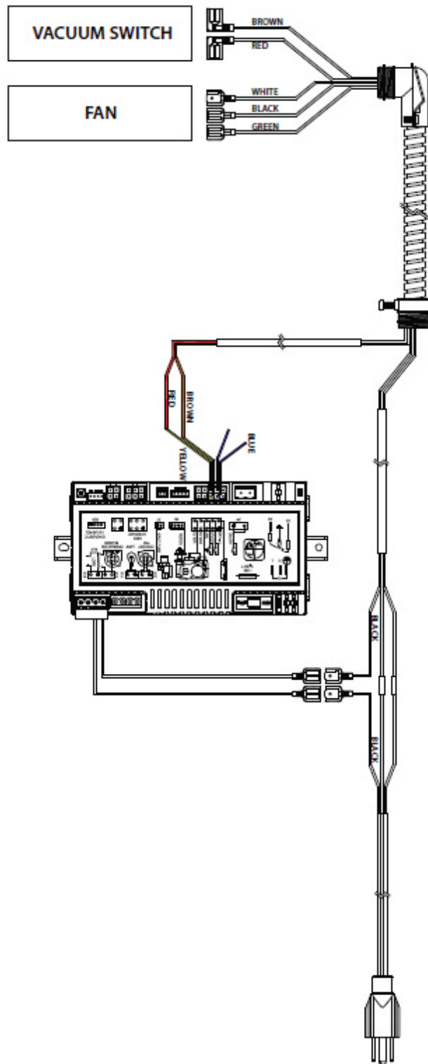
Figure 7.4 - Electrical Diagram
