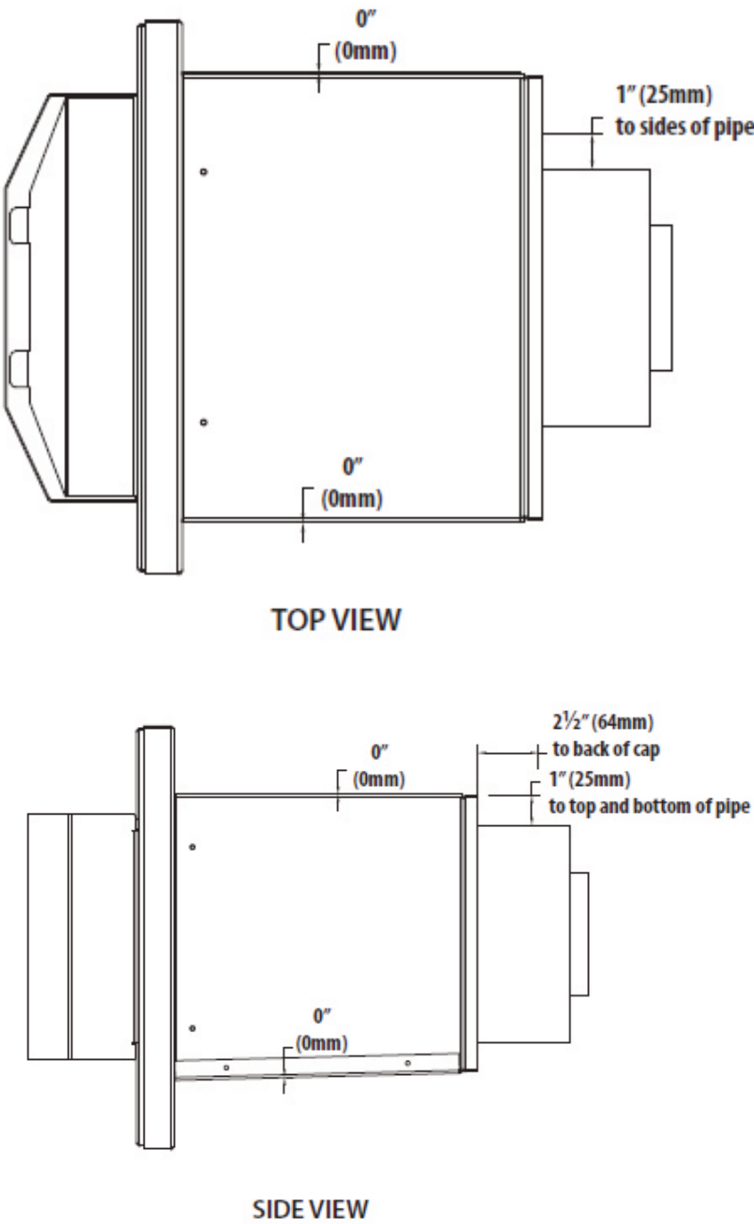
Figure 4.2 - Minimum Clearance to Combustibles
