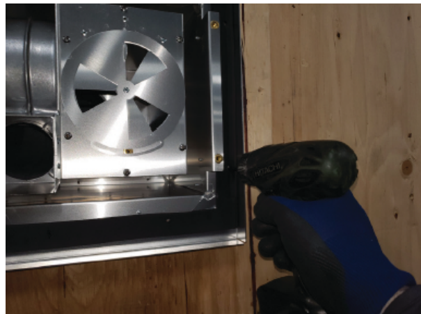
Figure 6.6 - Secure Power Vent to Exterior
