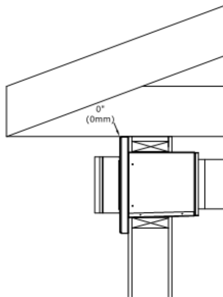
Figure 4.4 - Termination Top Clearance
