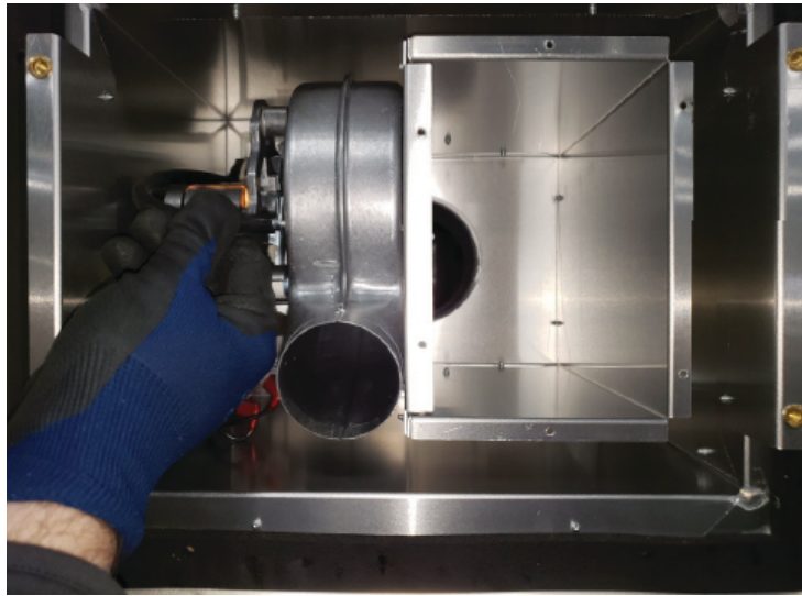
Figure 8.5 - Remove Vacuum Tube
