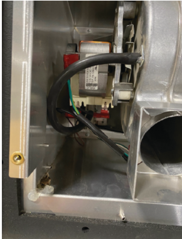
Figure 8.8 - Screws Securing Vacuum Switch Bracket
