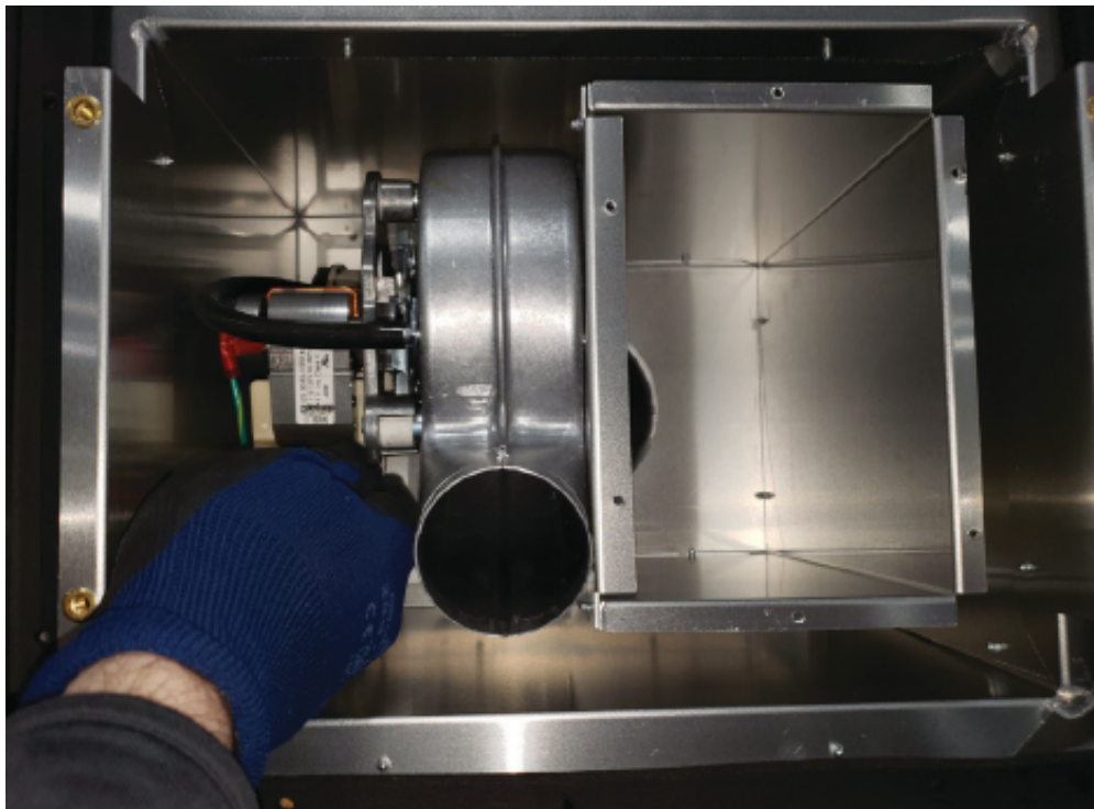
Figure 8.4 - Remove Live, Neutral, and Ground Wires
