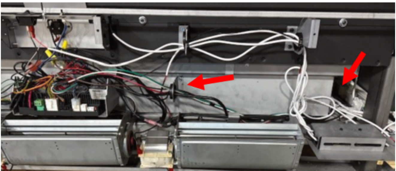
Figure 1.5 - LED Wiring Route
