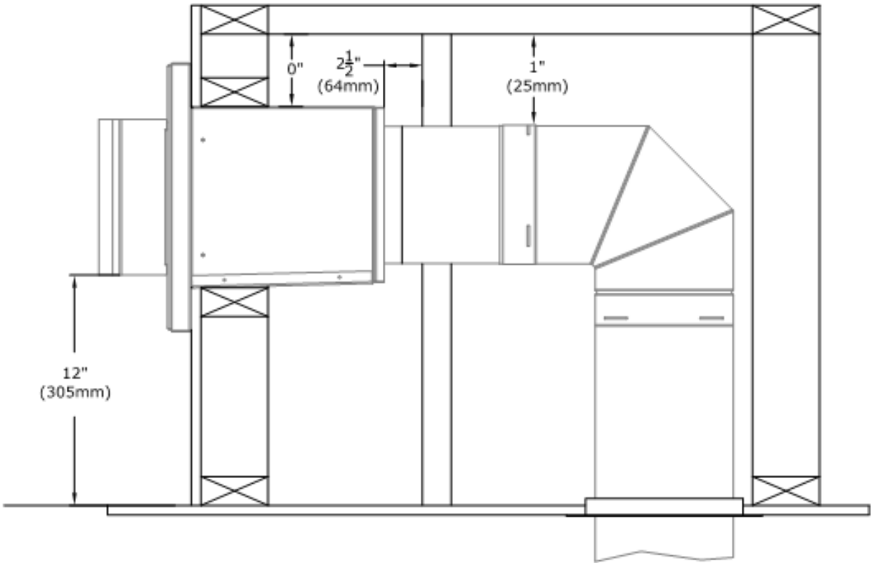
Figure 4.5 - Minimum Clearances for Rooftop Termination
